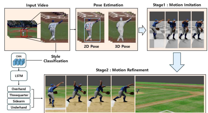
Figure 1: System overview
