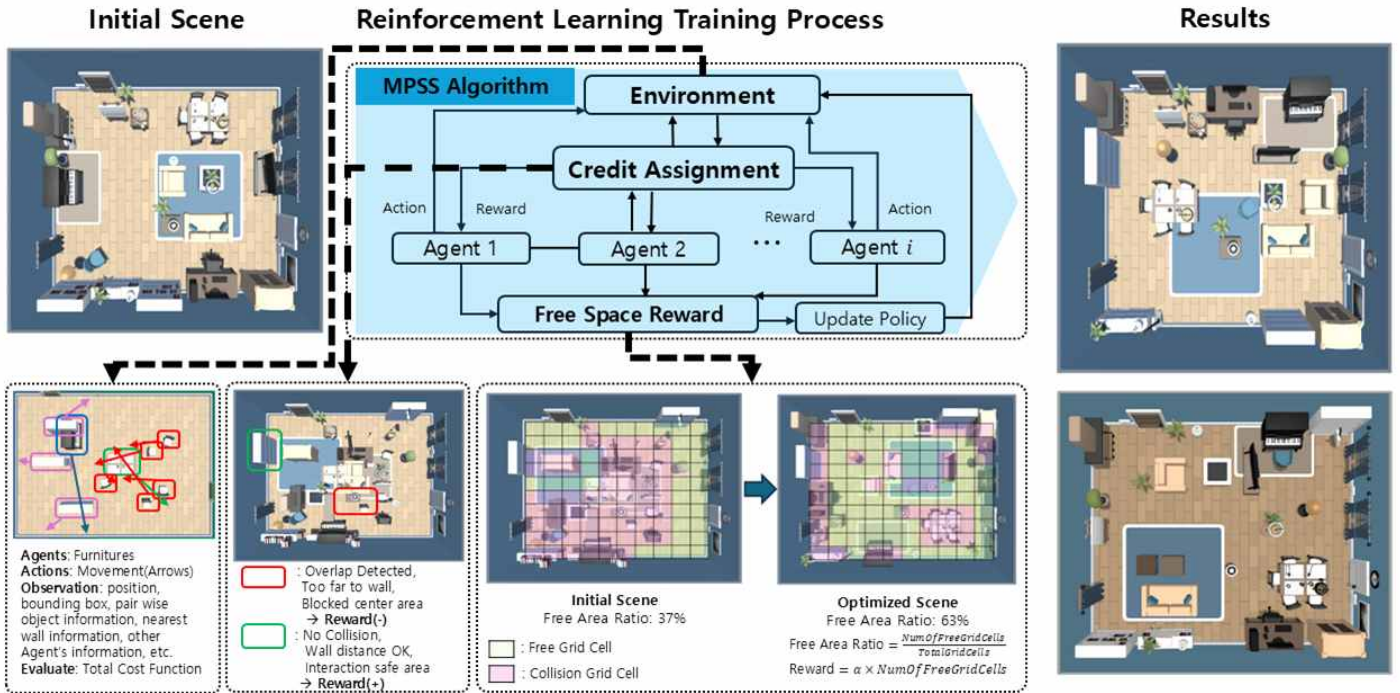
그림 1: Each furniture object is defined as an agent that observes its surroundings, selects movement actions, and receives rewards based on collision avoidance, relational constraints, wall proximity, and free space preservation. The environment incorporates a top-view grid for spatial reasoning and prior layout knowledge to guide optimization.
